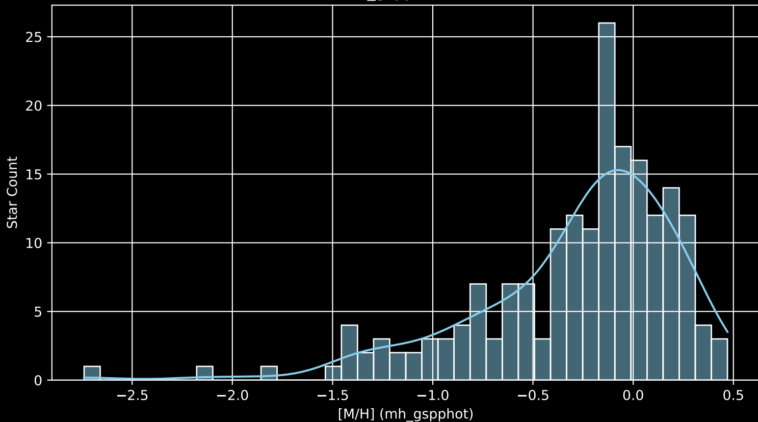
APOGEE DR17 Field: [K2_C11_005+07_btx [M/H] (mh_gspphot) (n= 192)
