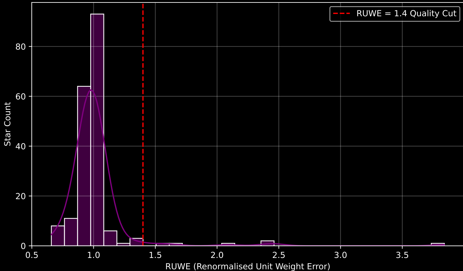
GAPOGEE DR17 Field [K2_C11_005+07_btx] RUWE Distribution (n= 192)
