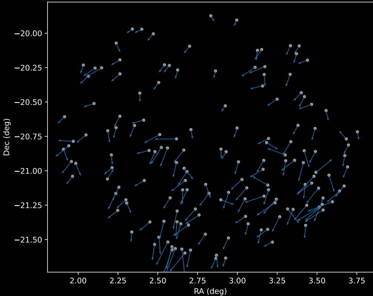
APOGEE DR17 Cluster 0 Proper Motion Vectors (n=154)
