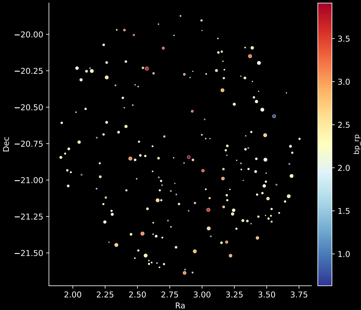
APOGEE DR17 Field: [K2_C11_005+07_btx] Stars: 193
