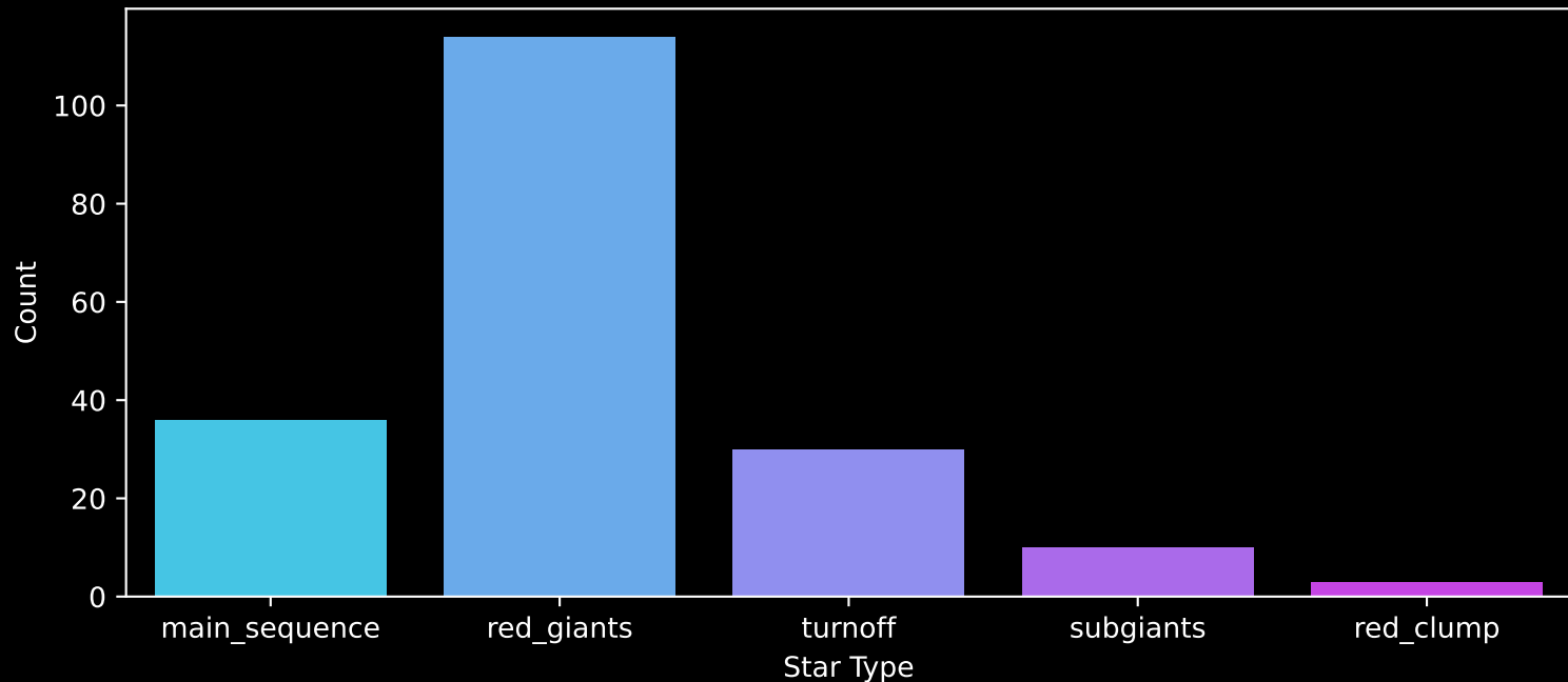
APOGEE DR17 Field: [K2_C11_005+07_btx] Count plot of Star Type
