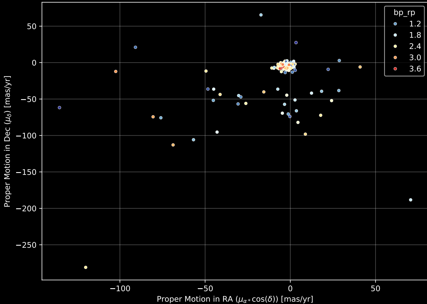
APOGEE DR17 Field: [K2_C11_005+07_btx] Proper Motion Diagram (n= 193)
