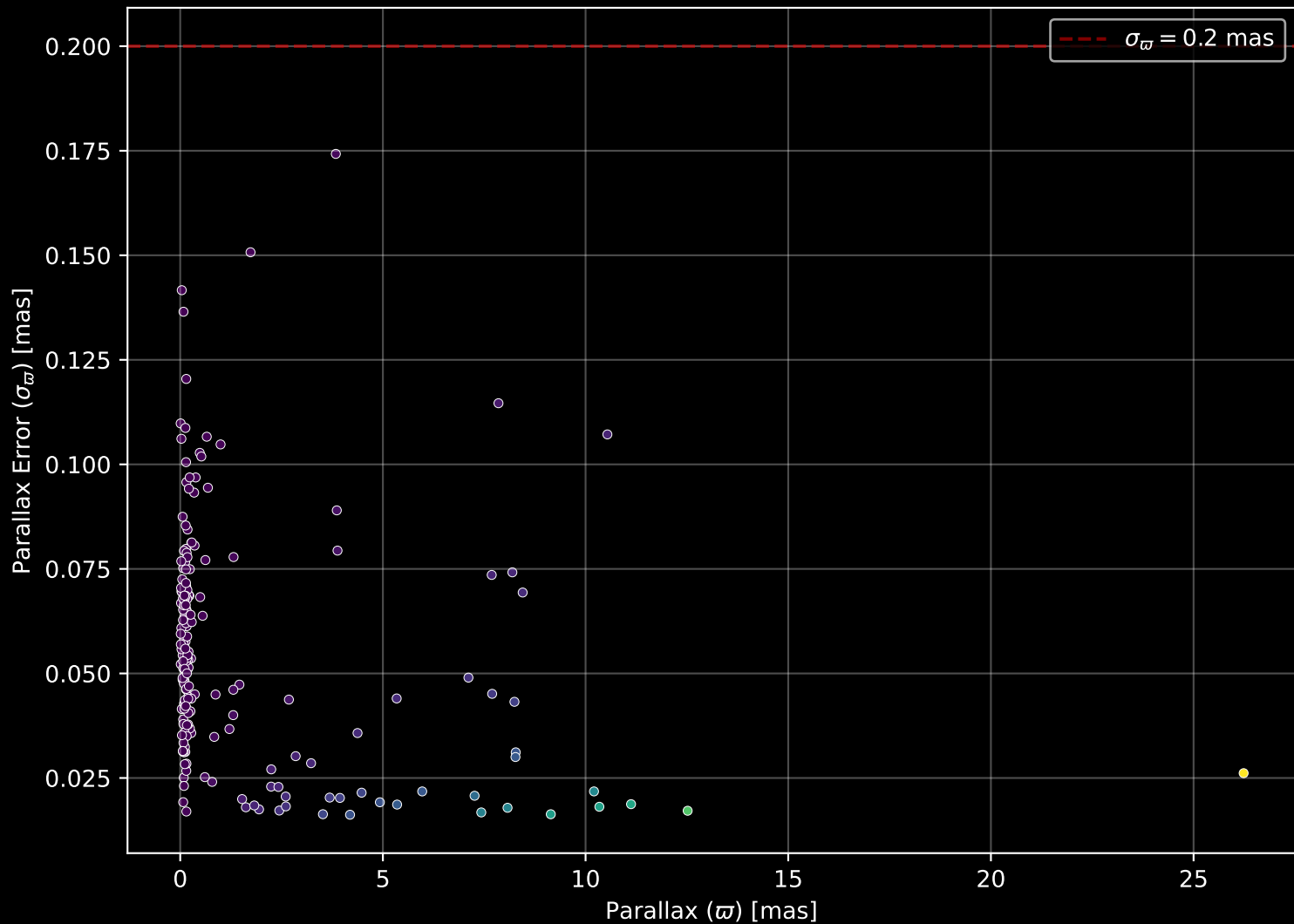
APOGEE DR17 Field: [K2_C11_005+07_btx] Parallax Quality (n= 193)
